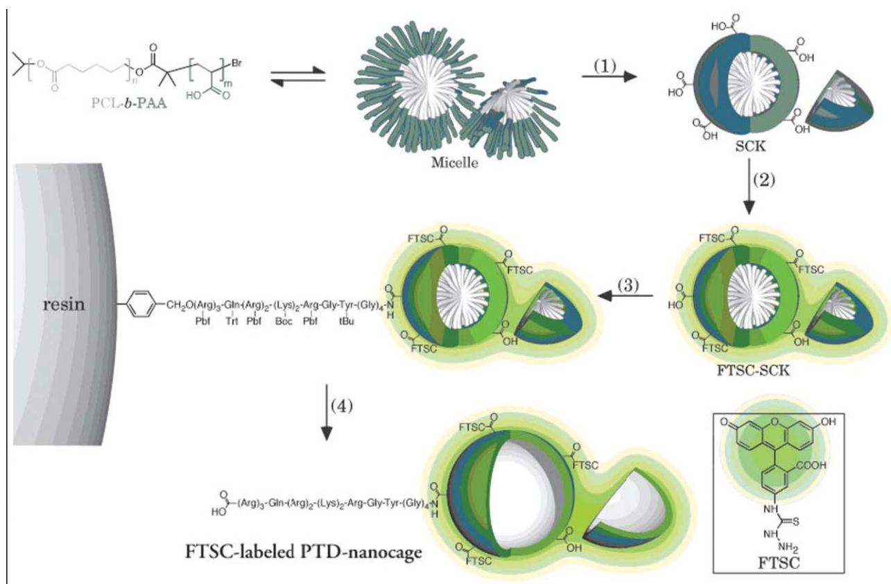
Fig. 10 Illustration of the synthetic strategy involving the coupling of a solid supported protein transduction domain (PTD) with a fluorescein labelled shell cross-linked nanoparticle, followed by cleavage from the support and core excavation. (Reproduced by permission from Ref. 36. Copyright 2001 American Chemical Society.)
