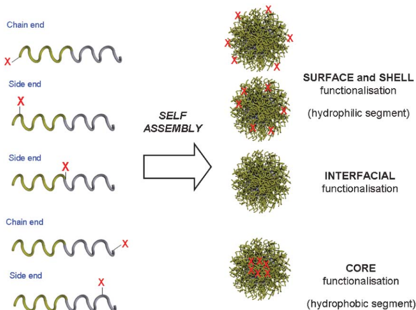
Fig. 5 Schematic to illustrate the possible locations of functionalisation within a spherical diblock copolymer micelle.
